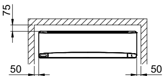
Minimum space requirements for installation
