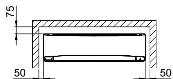
Minimum space requirements for installation
